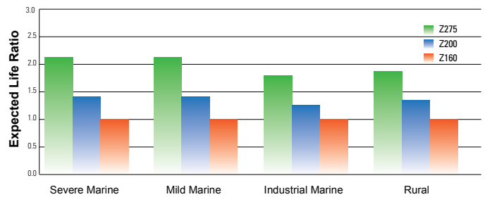
Galvanised Steel: Expected Life Ratio Comparison of Z275, Z200 and Z160 Coating Mass
