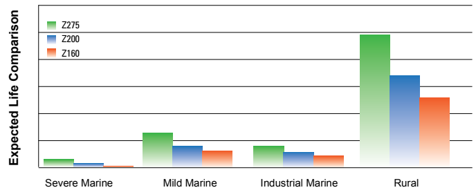
Galvanised Steel: Expected Life Comparison of Z275, Z200 and Z160 Coating Mass
